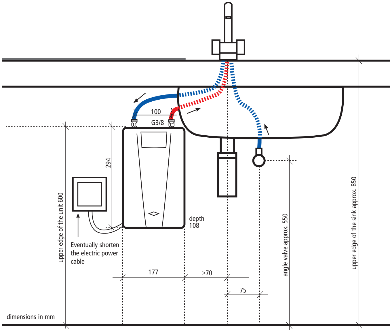
Example of an open-outlet installation with special tap.
