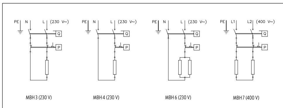
Fig. 7: "Circuit diagram"
