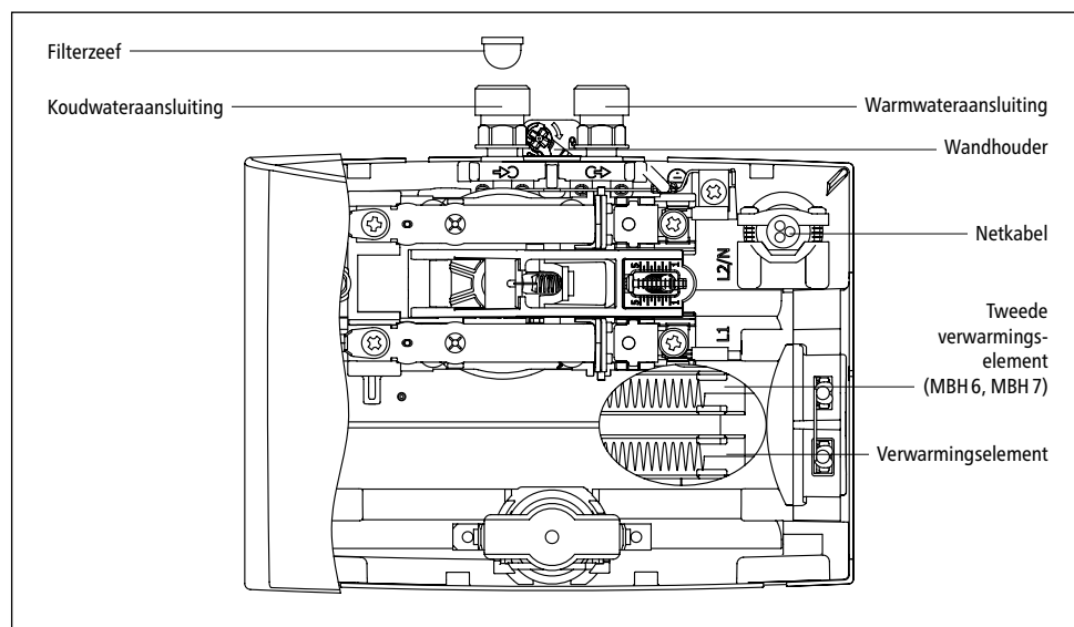
Afb. 12: "Reserveonderdelen"
